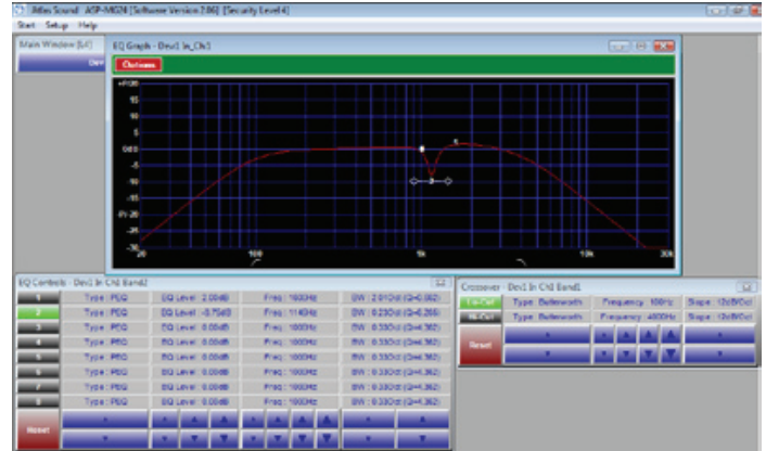
Equalizer Screen
