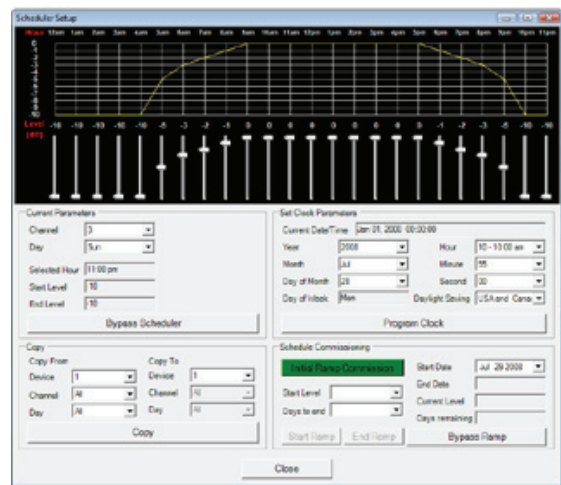
Scheduler Screen
