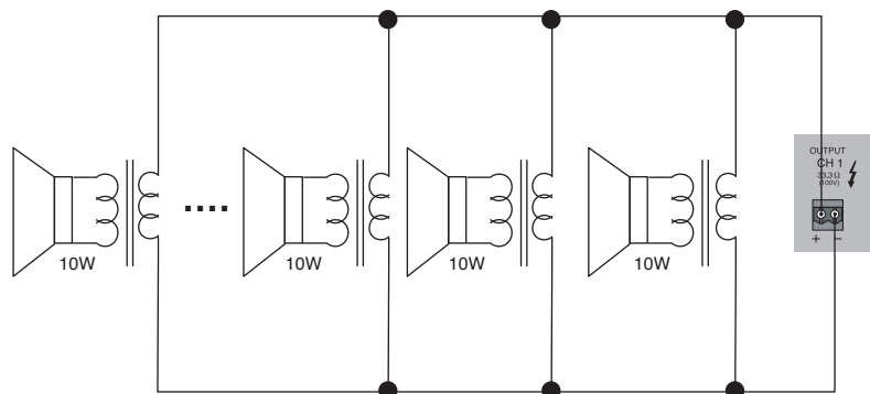
HIGH IMPEDANCE SPEAKER INSTALLATION (DPA-130DC)
