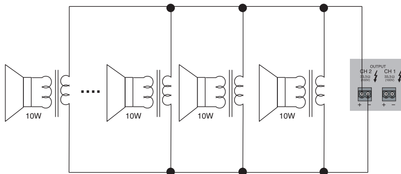
HIGH IMPEDANCE SPEAKER INSTALLATION (DPA-230DC)
