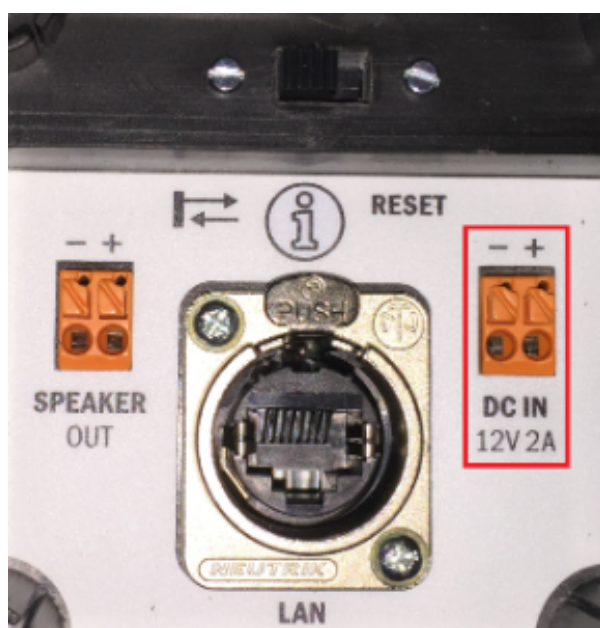
Figure: Power Supply Connection
