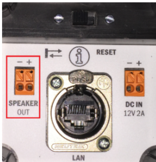
Figure: Loudspeaker Connection
