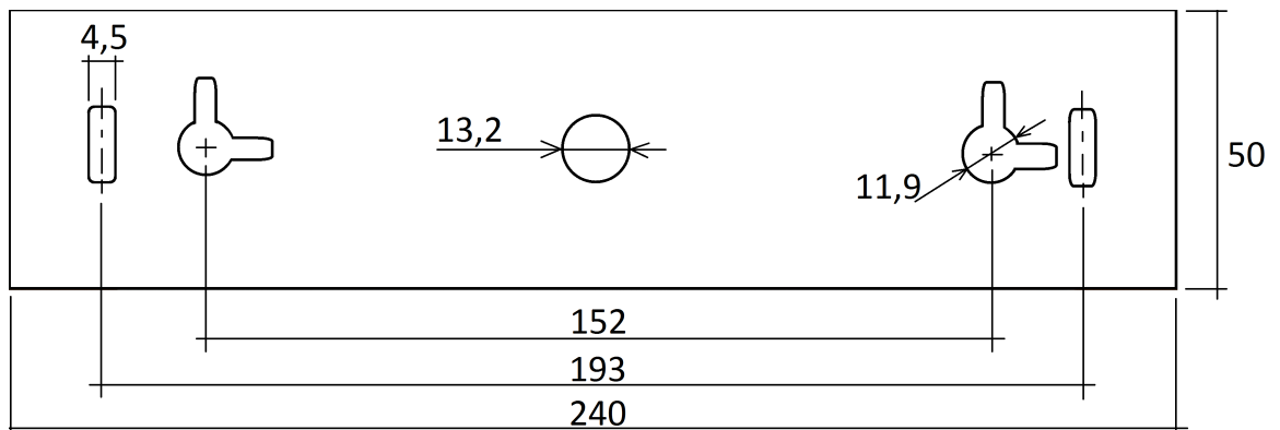
Figure: Mounting holes
