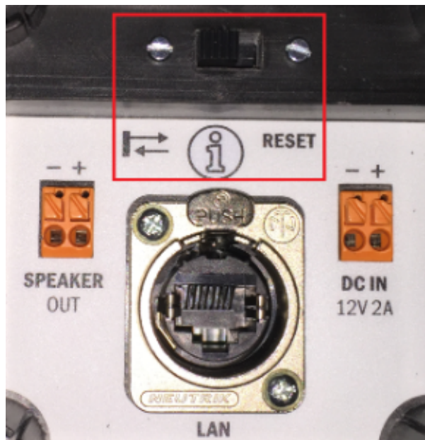
Figure: Reset with Static IP Address
